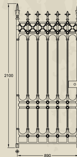
Stirling pedestrian gate (3 x 7ft, 142kg)
