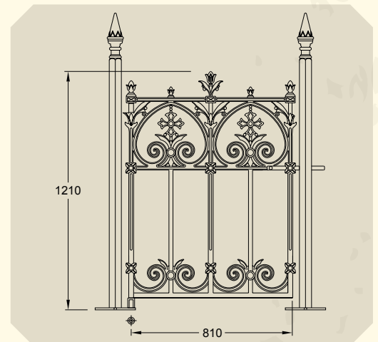
Terrace pedestrian gate (45kg) & Terrace pedestrian gate post (29kg)
