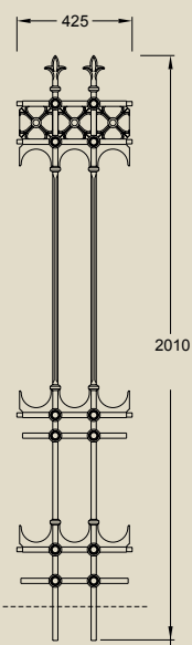
Stirling full height joining panel (18kg)
