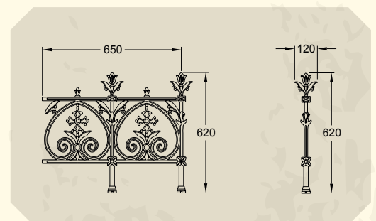
Terrace railing panel (36.5kg)
