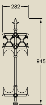
Stewart half height joining panel (10kg)
