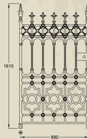
Stewart pedestrian gate (3ft, 117kg)
