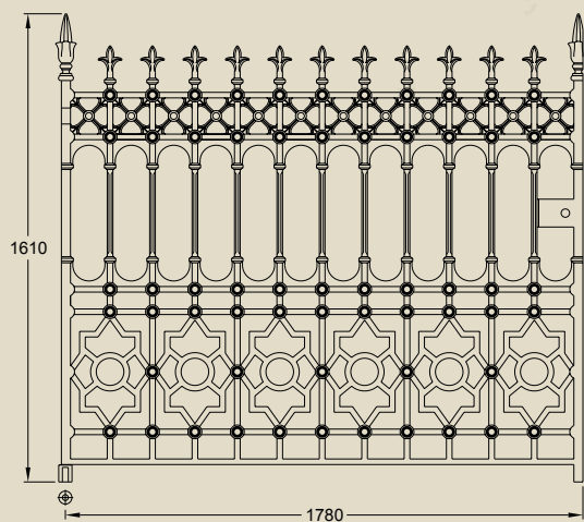
Stewart driveway gate leaf (12ft pair, 450kg)
