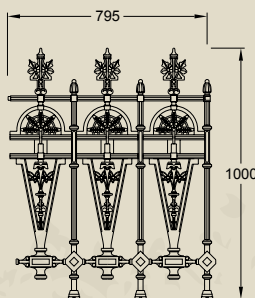
Gilberton railing panel (40kg)
